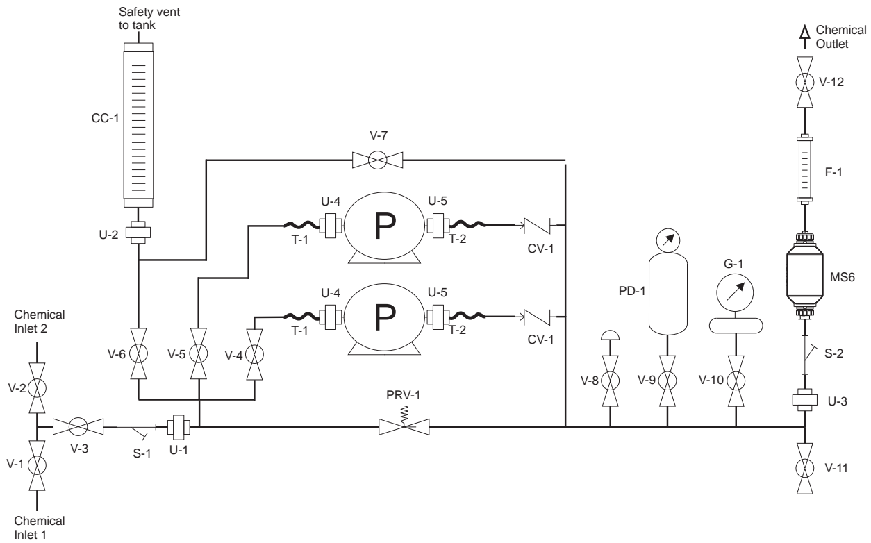
CFPS-2 P&ID
